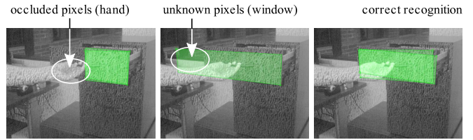
Fig. 4. Effect of the cost parameter for unknown and occluded pixels. Left: cost too high (1.0). Middle: cost too low (0.0). Right: good (0.2).
