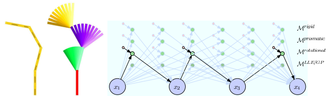
Figure 5: simulated yard stick consisting of 4 consecutive elements. Model selection correctly reveals the sequential chain.
