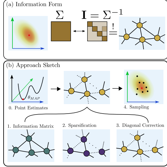
Figure 2. Illustration of the main idea and the pipeline sketch. We demonstrate that approximate Bayesian inference can work with the inverse covariance matrix - the information matrix. From its graphical interpretation ( Paskin, 2003 ), the diagonal elements represent the information content of the node while its off-diagonal elements represent the link between the nodes. Our approach is designed with this insight where we sparsify the weak links while keeping the information content of the node accurate.
