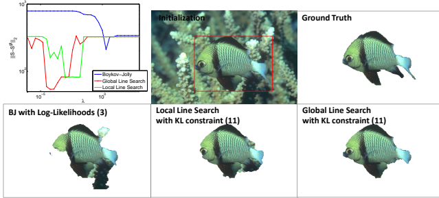
Fig. 6. Results for the “fish” from [7]. Note that Boykov-Jolly is very sensitive to \lambda .
