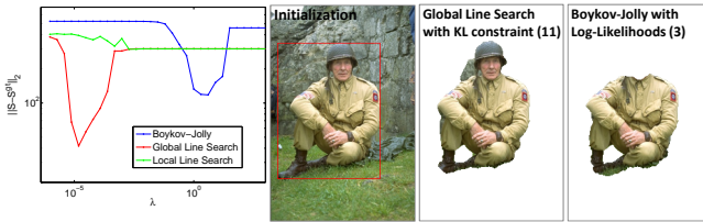
Fig. 7. Results for the “soldier” from [7]. The local-line search fails for all \lambda .
