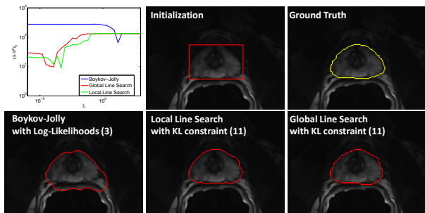
Fig. 5. Prostate midgland segmentation on T2W MRI, where fast and accurate segmentation is important to the planning of prostate cancer therapy. Both local and global line-search may obtain similarly good solutions for KL constraint (11), but the latter works for a wider range of \lambda .
