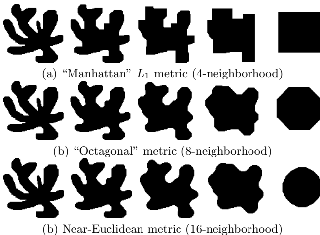
Fig. 2. Synthetic examples: line-search cuts can generate a “flow” of a 2D contour under energy E combining quadratic volume constraint (8) and boundary length for Manhattan (a), octagonal (b), and near-Euclidean (c) homogeneous metrics. Target volume is set to the initial volume of the shape. The last result is at convergence.
