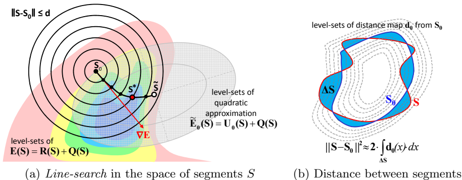
Fig. 1. Overview of line-search cuts . At each iteration, the algorithm finds global minimum S^* for energy E(S) along a curve approximating the line of gradient descent \nabla E from current solution S_0 . This follows the exact (global) line-search principle [17].
