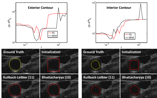
Fig. 9. Comparing the performance of Kullback-Leibler histogram constraint (11) (red) and Bhattacharyya histogram constraint (10) (black) in the task of 2D ultrasound carotid segmentation, with the outer wall shown on the left and lumen - on the right.
