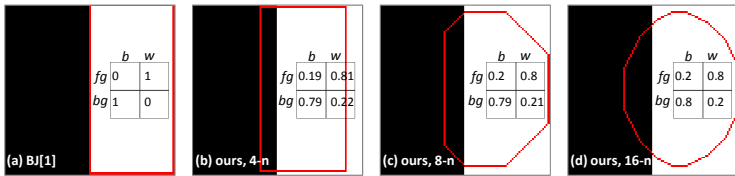
Fig. 3. Synthetic example: line-search cuts can match object and background intensity distributions to target distributions (b, w)_{fg} = (0.2, 0.8) and (b, w)_{bg} = (0.8, 0.2) by minimizing a combination of KL distance (11) and segmentation boundary length for Manhattan (b), octagonal (c), and near-Euclidean (d) homogeneous metrics. The result in (a) is the global minimum for Boykov-Jolly segmentation model with the standard linear log-likelihood term (3) using the same target distributions. When maximizing unary likelihoods (3) each pixel independently selects the most likely label regardless of the overall segment appearance. We use (a) to initialize line-search cuts in (b-d).
