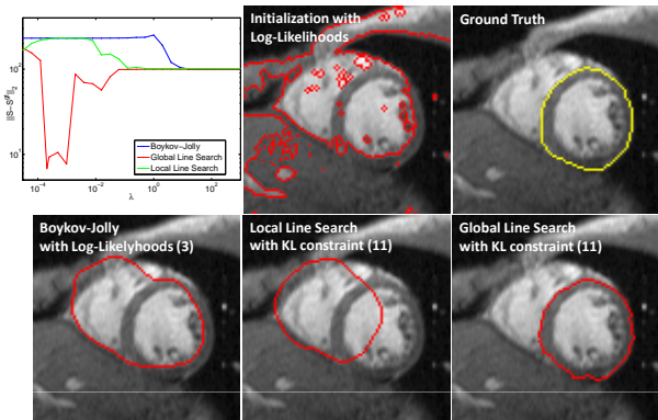
Fig. 4. Segmentation results for an MR image of a heart. Maximizing unary log-likelihoods (3) suffers from the same bias as in Fig. 3(a). Adding length-based regularization in Boykov-Jolly segmentation does not alleviate the problems of (3). The local-line search using more powerful KL constraint (11) gets stuck in a local minimum, whereas the global line-search makes large moves overcoming many weak local minima.
