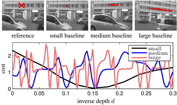
Figure 3. Variable Baseline Stereo: Reference image (left), three stereo images at different baselines (right), and the respective matching cost functions. While a small baseline (black) gives a unique, but imprecise minimum, a large baseline (red) allows for a very precise estimate, but has many false minima.
